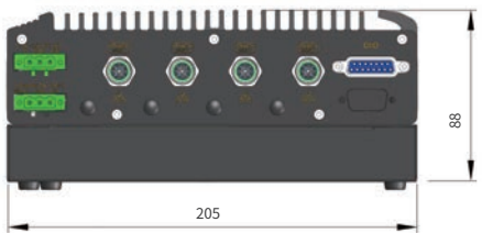
Nuvo-2611VTC Nuvo-2612VTC
