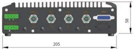
Nuvo-2610VTC
